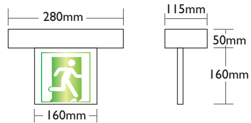
Size of CX-LED-165-P-OPL
