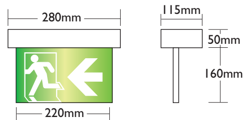
Size of CX-LED-220-P-OPL
